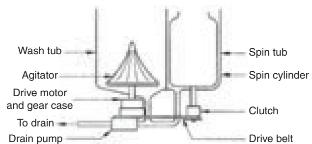
Fig. 4.20 Construcion diagram
