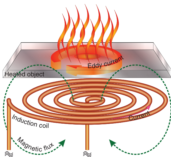
Fig. 3.6 Induction stove
