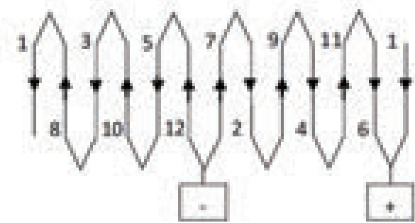
Fig. 9.9 Winding-commutator connection
