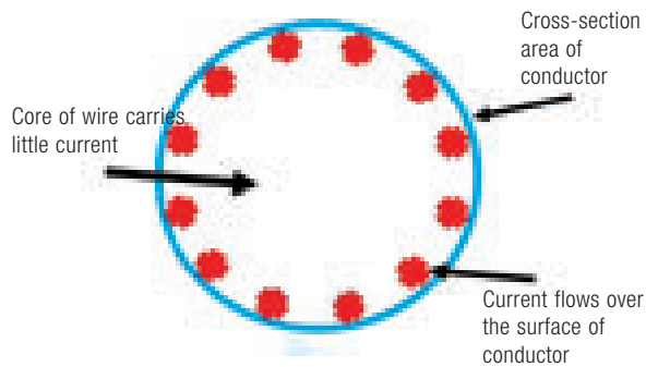
Fig. 1.8 Skin effect
